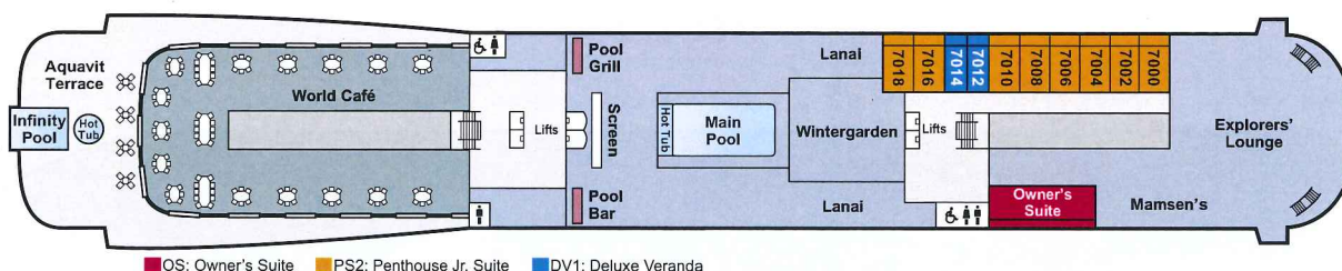
DECK 7
